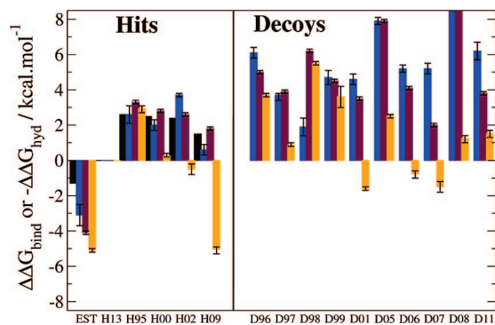
Figure 6. Discrimination of hits from decoys by plotting hydration free energies or Chemscore binding energies. In black, the experimental IC_{50} s converted to relative binding affinities with eq 6, in blue, the negative of the hydration free energies predicted by explicit solvent simulations, in maroon, the negative of the hydration free energies predicted by revised implicit solvent simulations, and in orange, the binding energies predicted by Chemscore. The relative hydration free energy of D08 is off-scale and stands at 38.4 \pm 0.5 and 34.6 \pm 0.1 kcal·mol -1 for the simulations in explicit and implicit solvent, respectively. All the figures are relative to ligand H13. The error bars show one standard error.
